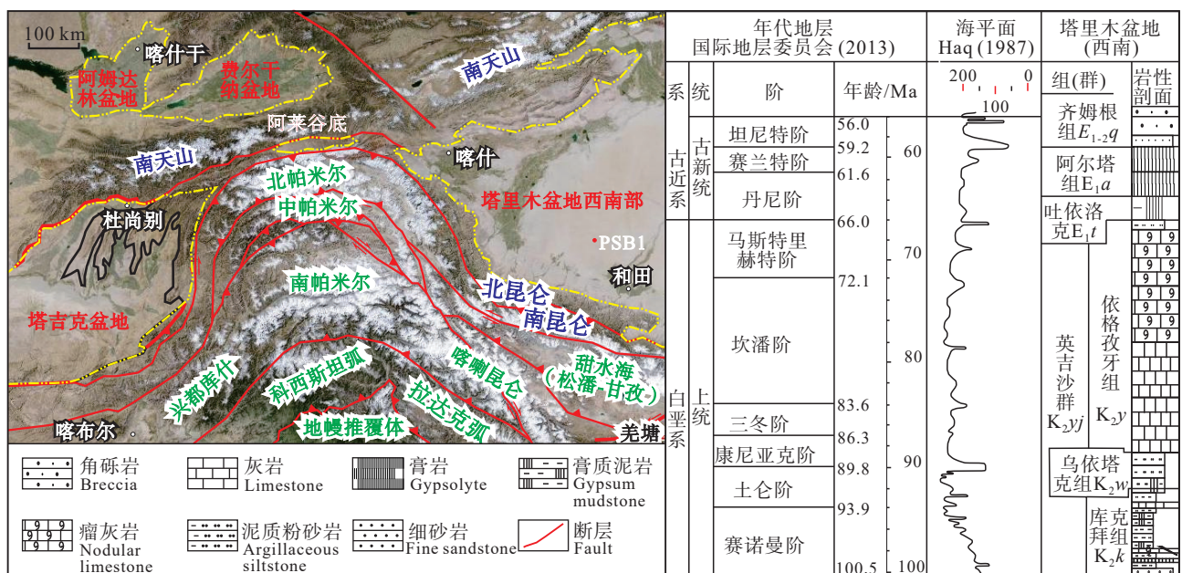
图 1 塔里木盆地西南部构造位置及地层发育特征 Fig.1 Tectonic location and stratigraphic development in the southwestern Tarim Basin
