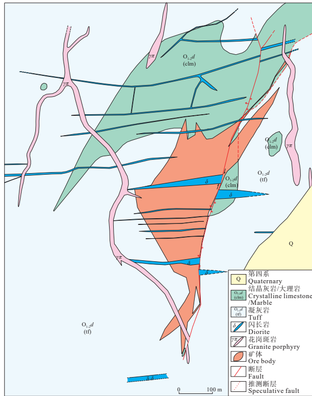
图2 二道河铅锌银多金属矿矿区地质简图 Fig.2 Sketch map of the Erdaohe Pb-Zn-Ag polymetallic deposit
