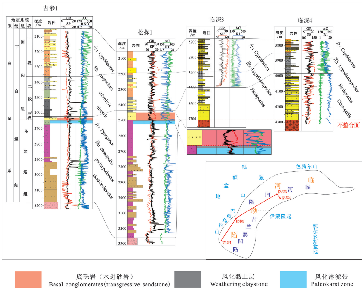
图3 临河坳陷吉参1-松探1-临深3-临深4连井剖面 Fig.3 Profile of Linhe Depression Jishen1-Songling1-Linshen3-Linshen4 Union well
