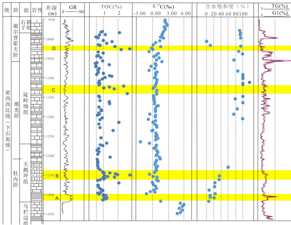
图 2 湘新地 4 井下石炭统岩性、伽马、总有机碳, \delta^{13}\text{C} 、含水饱和度与气测值 (图例同图 3) Fig. 2 lithology, gamma, TOC, \delta^{13}\text{C} , water saturation and gas content of the Lower Carboniferous at well of Xiangxindi 4 (The lithology legend is shown in Figure 3)
