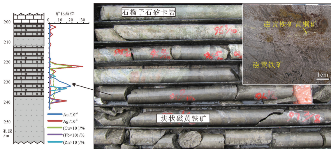
图8 甲玛矿床 ZK8806 含 Au 磁黄铁矿手标本和柱状图 Fig.8 Hand specimen and column diagram of Au bearing pyrrhotite in Jiama deposit
