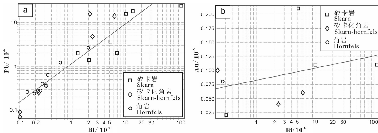
图7 甲玛矿床磁黄铁矿 Bi-Pb 和 Bi-Au 关系图 Fig.7 Bi vs. Pb and Bi vs. Au diagrams of pyrrhotite in Jiama deposit (legend same as Fig.4)
