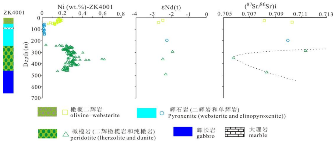
图 8 石头坑德矿区 ZK4001 岩相、镍含量与 \epsilon Nd(t) 、 (^{87}Sr/^{86}Sr)_i 的对应关系(Zhang et al., 2018) Fig. 8 The relationship of nickel content with \epsilon Nd(t) and (^{87}Sr/^{86}Sr)_i in Shitoukengde Cu-Ni deposit (Zhang et al., 2018)
