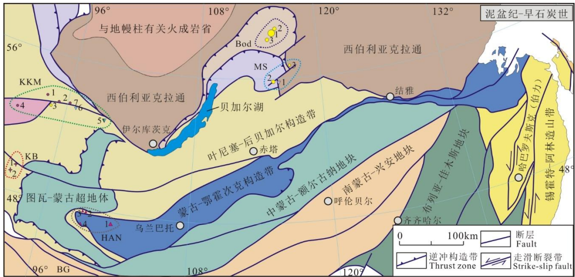
Bod 博代宾斯基Au成矿带 Bodaibinskiy Au metallogenetic belt MS 穆伊斯基Au-Sn成矿带 Muiskiy Au-Sn metallogenetic belt HAN 杭爱Fe-Mn成矿带 Hangai Fe-Mn metallogenetic belt KB 卡勒赞-博尔歌德Nb-Ta-Zr成矿带 Khalzan-burged Nb-Ta-Zr metallogenetic belt KKM 基日-赫姆Au-Cu-Be-Mo-Li成矿带 Kizhi-Khem Au-Cu-Be-Mo-Li metallogenetic belt
