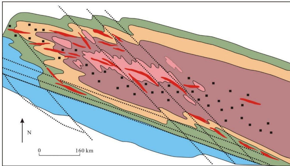
钙质石灰岩、钙质粉砂岩、砂岩 Carbonaceous limestone, calcareous siltstone, and sandstone 含碳千枚岩-粉砂岩 Carbonaceous phyllite-siltstone 金-石英-硫化物晕 Halo of Au-quartz-sulfides 强烈黄铁矿化带 Zone of intense pyritic alteration 粉砂岩、石英长石云母砂岩 Siltstone and quartz-feldspar-mica sandstone 含碳石英绢云母粉砂质页岩 Carbonaceous quartz-sericite silty shale 金矿体 Au ore body 断裂带 Fault
