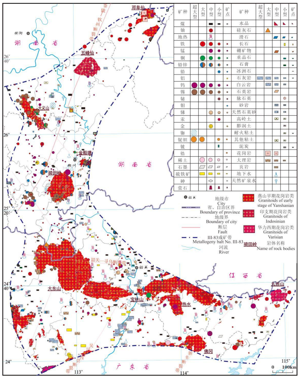
图2 南岭成矿带中段区域地质矿产图 Fig. 2 Regional Geological and mineral resources Map of the middle part of the Nanling metallogeny belt
