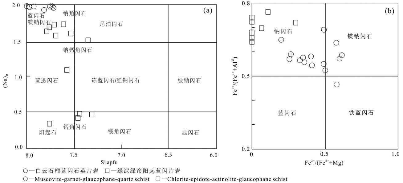
图4 景洪大勐龙勐宋坝地区白云石榴蓝闪石英片岩和绿泥绿帘阳起蓝闪片岩中闪石族矿物成分图解(根据Leak et al., 1997) Fig.4 Mineral component diagrams of amphiboles in the muscovite-garnet-glaucophane-quartz schists and chlorite-epidote-actinolite-glaucophane schists from the Damenglong-Mengsongba area, Jinghong City (after Leake et al., 1997)
