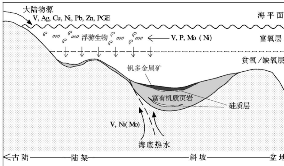
图9 沉积型钒多金属矿成矿模式图 (据施春华等, 2013; 韩善楚, 2013 修改) Fig.9 Metallogenic model of sedimentary polymetallic V-polymetallic deposits
