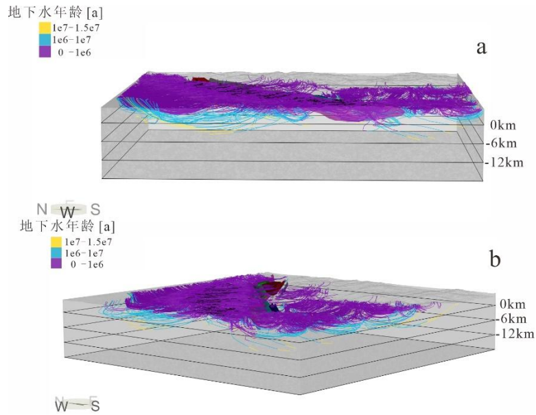
图 11 补给高程高于 5500m 以上地下水流线年龄的模拟结果：(a) W 向，(b) SW 向 Figure.11 Groundwater streamline agesimulation results with recharge elevation above 5500m: (a)W direction; (b)SW direction.
