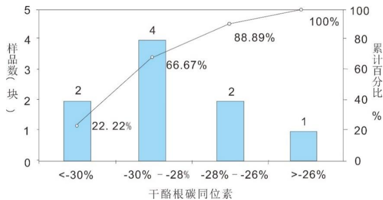
图 3 鄂宜地 2 井水井沱组干酪根 \delta^{13}\text{C}_{\text{org}} 值统计直方图 Fig.3 Statistical histogram of kerogen \delta^{13}\text{C}_{\text{org}} value of Shuijingtuo Formation in Eyidi 2 well
