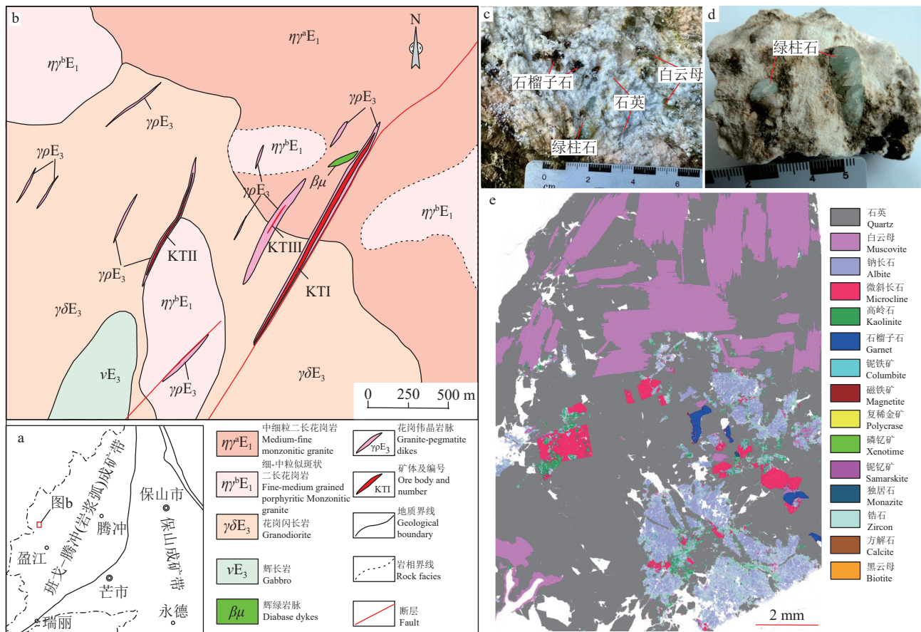
图1 腾冲成矿带构造示意图(a)、卡场地区地质图(b)、花岗伟晶岩野外及标本照片(c~d)、矿石TIMA照片(e) Fig.1 Sketch map of Tengchong metallogenic belt (a), geological map (b), pegmatite field photos (c~d) and TIMA (e) of the Kachangrare polymetallic deposit
